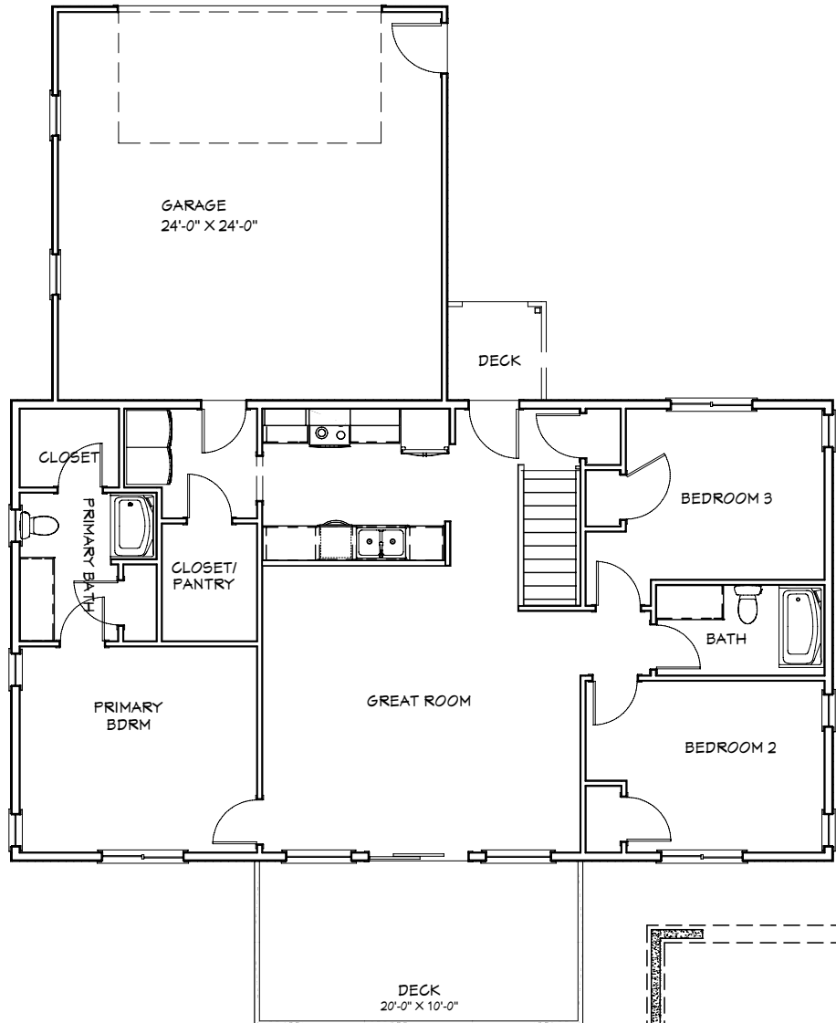
1st Floor
