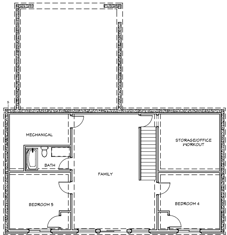
Walkout Basement
