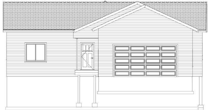
Street Elevation
