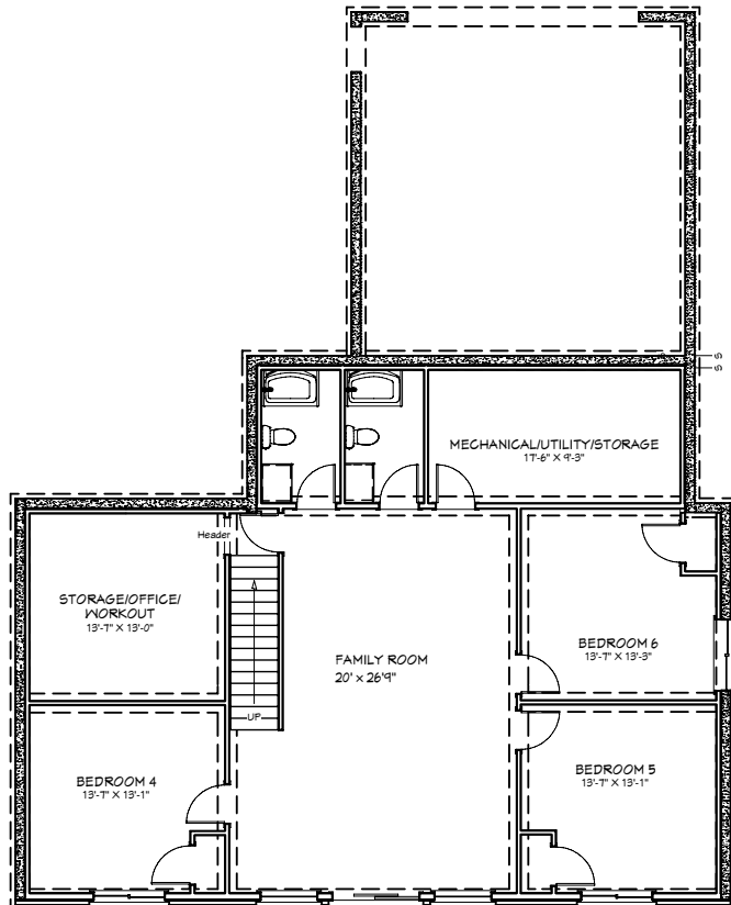
Walkout Basement
