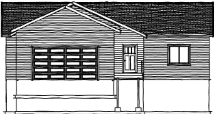
Street Elevation
