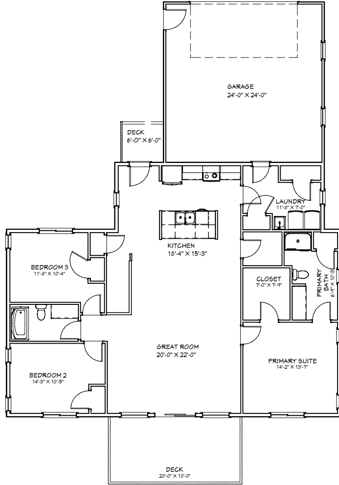
1st Floor
