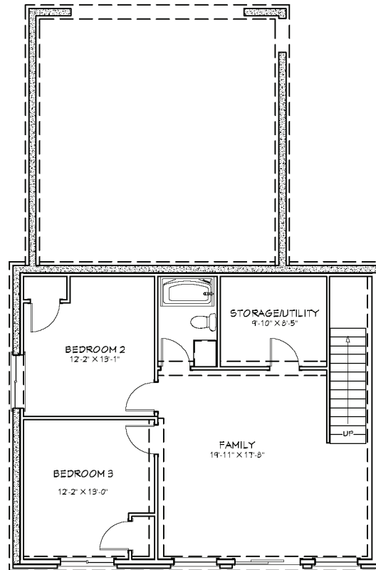
Walkout Basement
