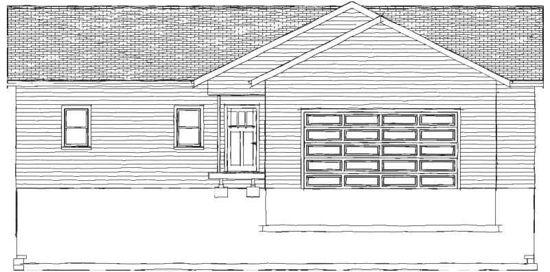
Street Elevation
