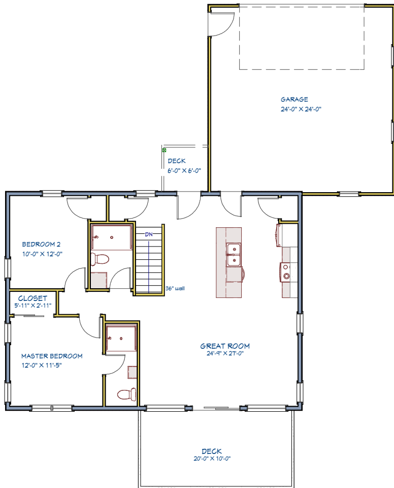
1st Floor
