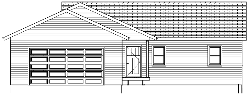
Street Elevation
