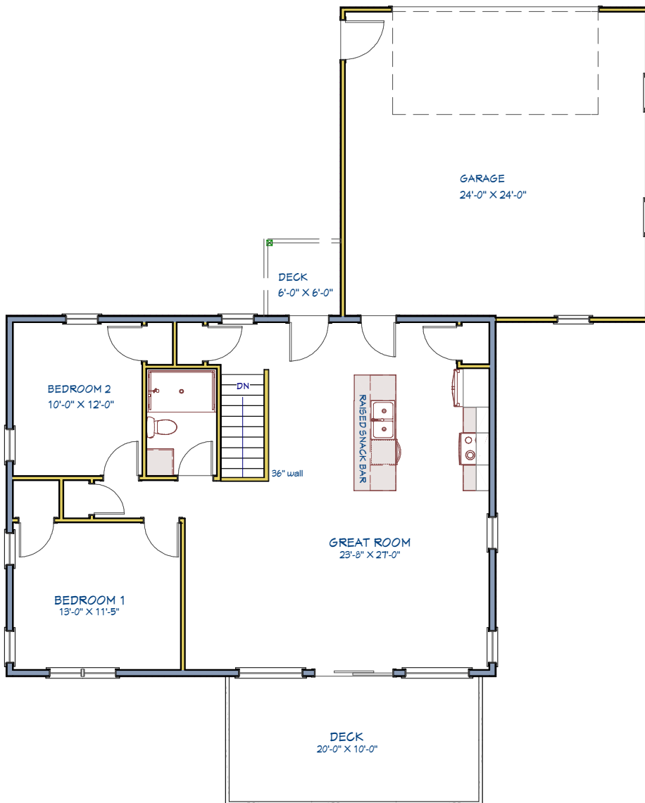
1st Floor
