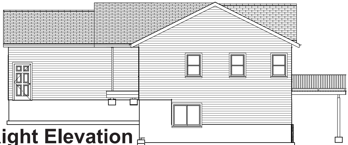
Left Elevation
