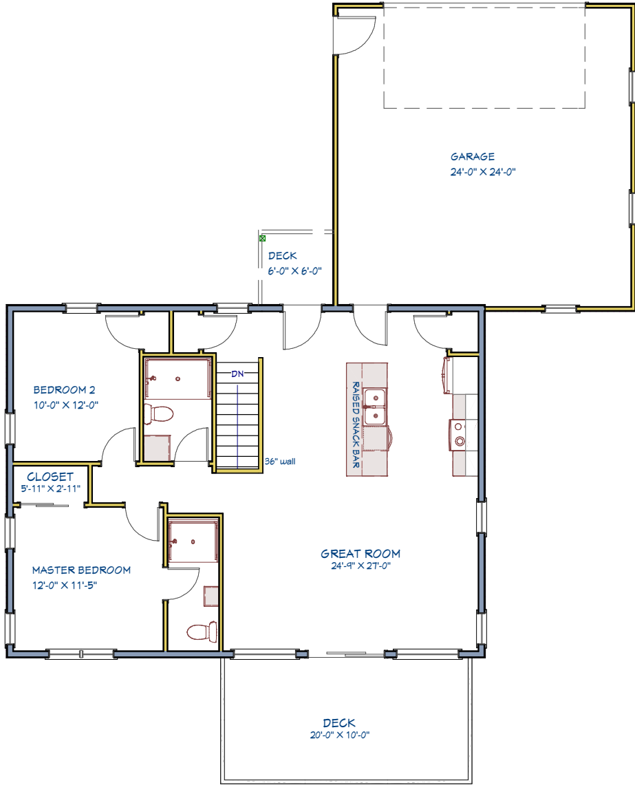
1st Floor
