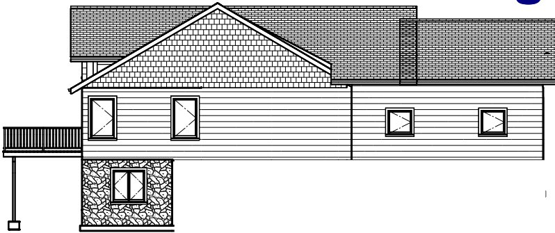
Left Elevation
