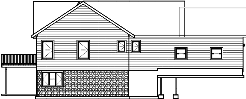
Left Elevation
